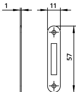
A1004 Piastrina Striker plate
