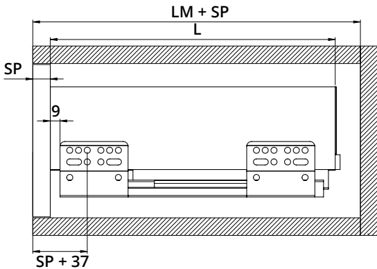
Pannello spessore: 16 mm Panel thickness: 16 mm
