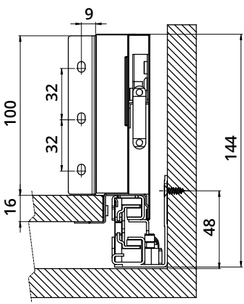
Vista retro / Back view
